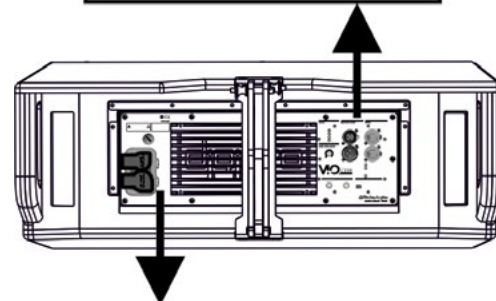
INPUT, OUTPUT AND CONTROL SECTION
