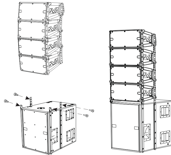
In appoggio con kit staffe Groundstack with kit stirrups
