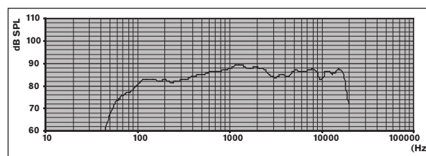
Frequency response
